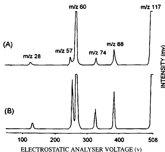
FIGURE 2 MIKE spectra of (A) molecular ion for 1 (B) fragment ion at m/z 117 for 6
