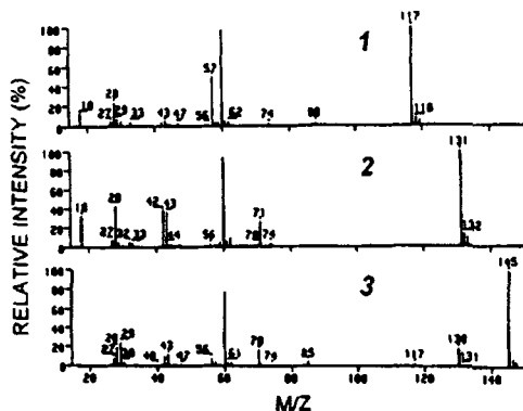
FIGURE 1 70 eV EI mass spectra of 1-3
